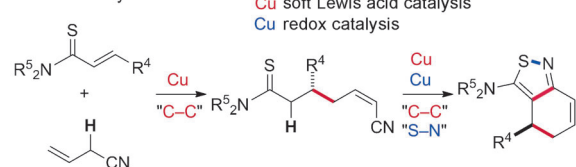
Scheme 1. Formation of isothiazoles.
